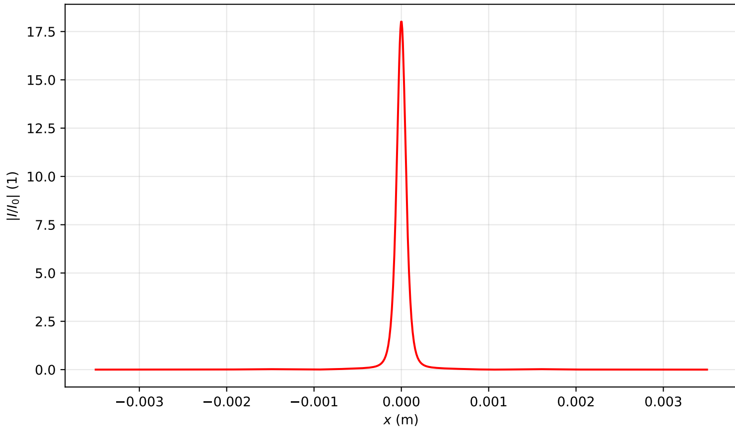
Intensity profile I(x, y = 0, z = 2.627)/I_0 , P_{in}=2.0P_{cr} , artificial time
